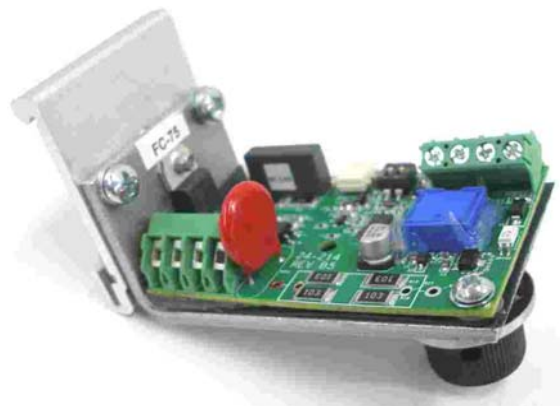
2. Remove Rodix Nameplate and Screw FC-75 to bracket
